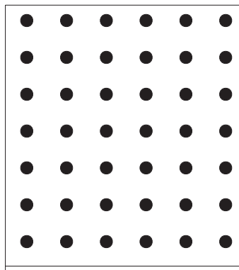
Round Hole Square Large Diameter 3.1mm Pitch 8mm Perforated area 11.5% Maximum width 600mm
