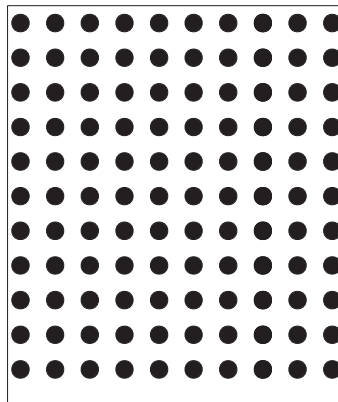
Round Hole Square Small Diameter 2.4mm Pitch 5mm Perforated area 18% Maximum width 800mm
