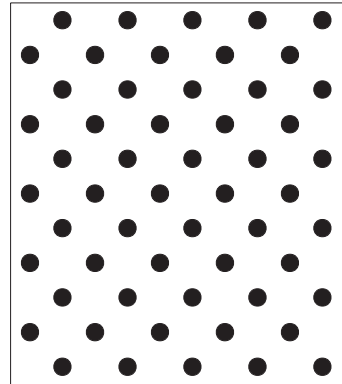
Round Hole Diamond Small Diameter 2.4mm Pitch 9.5mm Perforated area 11% Maximum width 600mm
