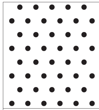
Round Hole Diamond Large Diameter 3.1 mm Pitch 8mm Perforated area 11.25% Maximum width 600mm
