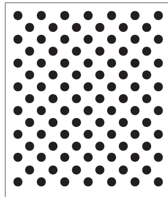
Round Hole Diamond Medium Diameter 2.5mm Pitch 7mm Perforated area 20.1% Maximum width 800mm
