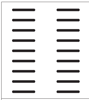
Slotted Large 12.7 mm x 1.9mm Pitch 19mm x 5.7mm Perforated area 19.5% Maximum width 600mm
